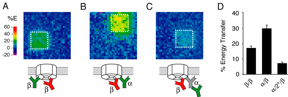
Figure 3. Detection and characterization of Sec61 complex oligomerization in situ. (A–C) Direct comparisons of FRET efficiencies to Sec61 \beta_{C_{y5}} from three different donor antibodies: Sec61 \beta_{C_{y3}} (at a ratio of 1:8; A), Sec61 \alpha_{C_{y3}} (B), and 2^{\circ}C_{y3} bound to unlabeled anti-Sec61 \alpha (C). (D) Quantitation (mean \pm SD; n = 10 ) of the comparisons from A–C are shown.
