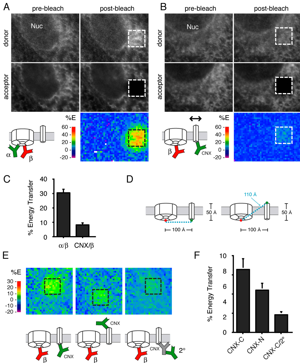
Figure 2. Discrimination of protein proximities with low nanometer resolution. (A and B) MDCK cells were double labeled with Sec61 \alpha_{\text{Cy3}} and Sec61 \beta_{\text{Cy5}} (A) or CNX \text{Cy3} and Sec61 \beta_{\text{Cy5}} (B) and analyzed for FRET as in Fig. 1 E. (C) Quantitative analysis of FRET between the antibody configurations shown in A and B. The antibody pair is indicated on the x-axis, with Sec61 \beta_{\text{Cy5}} serving as the acceptor in each case. Each bar represents the mean \pm SD ( n = 10 ), with statistically significant differences ( P < 0.01 using t test) being observed between the two conditions. (D) Illustration of the relative difference in distance for antibodies on the cytoplasmic and luminal sides of CNX. Note that moving the donor antibody to the other side of an \sim 5 -nm-thick membrane changes the distance to the acceptor antibody by only \sim 1 nm in this example. (E) Representative energy transfer maps of FRET to Sec61 \beta_{\text{Cy5}} from Cy3-labeled antibodies in three different positions. The left and middle panels used directly conjugated anti-CNX antibodies against the COOH and NH _2 terminus, respectively. The right panel used 2 ^\circ \text{Cy3} bound to an unlabeled anti-CNX COOH terminus antibody. The color scale is different than in A and B to enhance visualization of differences between the energy transfer maps. (F) Quantitative analysis of FRET between the antibody configurations shown in E. The donor antibody is indicated on the x-axis, while Sec61 \beta_{\text{Cy5}} served as the acceptor in each case. Each bar represents the mean \pm SD ( n = 10 ), with statistically significant differences ( P < 0.01 using t test) being observed between any two conditions.
