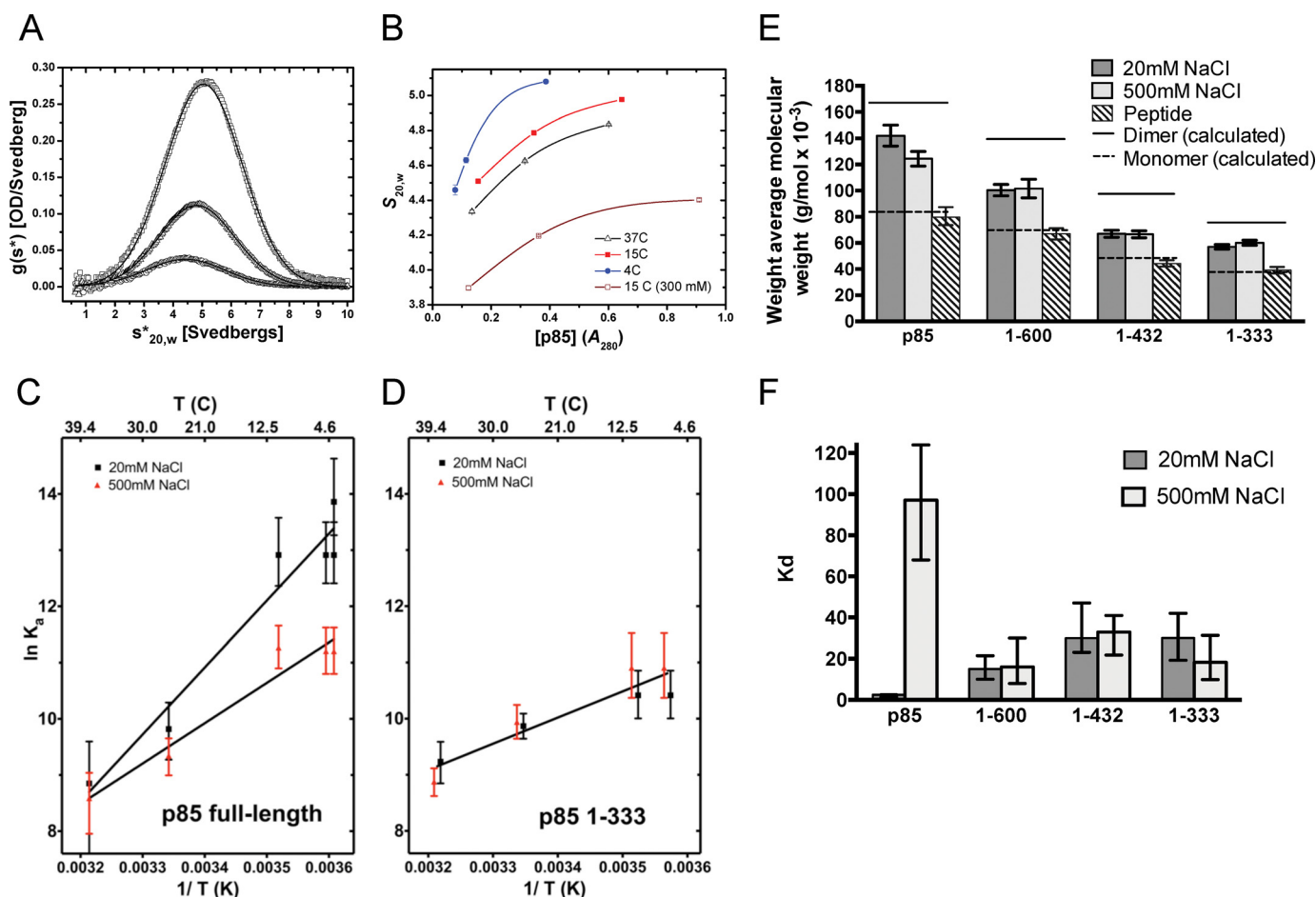
FIGURE 3. p85 \alpha dimerization in vitro measured by AUC. A , sedimentation coefficient distribution, g(s^*) , obtained from sedimentation velocity analysis of p85 \alpha at three concentrations (1.2, 3.6, and 9.5 \mu\text{M} ) in 20 mM NaCl-containing buffer at 4 ^{\circ}\text{C} . All sedimentation coefficient ( S , in Svedberg units) values presented in the paper have been corrected to 20 ^{\circ}\text{C} and the density of water ( s_{20,w} ) to allow comparison of data from experiments performed in different buffers and temperatures. B , plot of sedimentation velocity data showing S as a function of p85 \alpha concentration (absorbance at 280 nm) at 4, 15, 37, and 15 ^{\circ}\text{C} in 300 mM NaCl-containing buffer. C and D , van't Hoff plots relating the association constant ( K_d ) determined by sedimentation equilibrium analysis as a function of temperature for full-length p85 \alpha ( C ) and p85 \alpha (1–333) ( D ) in 20 and 500 mM NaCl-containing buffer. E , weight average molecular weights obtained from sedimentation equilibrium analysis of p85 \alpha and corresponding fragments in buffer containing either 20 mM NaCl or 500 mM NaCl and at 500 mM NaCl in the presence of 250 \mu\text{M} SH3-binding peptide. Solid and dashed lines , dimer and monomer molecular weights calculated from sequence, respectively. F , dissociation constant ( K_d ) values for each p85 \alpha construct in low and high salt, derived from fitting sedimentation equilibrium data to a monomer-dimer association model. Values are represented with joint confidence intervals of one S.D.
