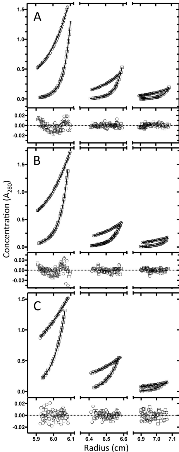
FIGURE 4. Sedimentation equilibrium analysis of p85 \alpha at 10 °C. The graphs show the distribution of p85 \alpha protein concentration during sedimentation equilibrium analysis at 10 °C obtained by measuring the absorption at 280 nm versus the radial distance from the center of the rotor. Three concentrations of full-length p85 \alpha were analyzed (1.2, 3.6, and 9.6 \mu M). The equilibrium protein concentration distributions measured at each of the two rotor speeds are shown ( top curve , 8,000 rpm; bottom curve , 16,000 rpm) with the best global fit to a monomer-dimer association model shown as the solid line in 20 mM NaCl (A) and 500 mM NaCl (B) and fit to the weight average molecular weight of a single species in 500 mM NaCl in the presence of proline-rich peptide (C). The residuals for the fit are shown by the symbols along the dotted line at 0.0.
