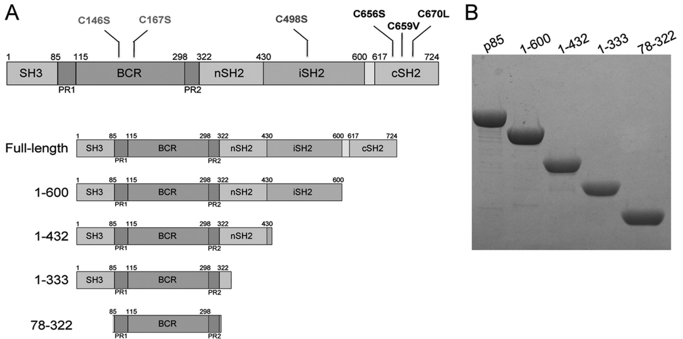
FIGURE 1. Cysteine-free p85 \alpha and fragments. A , the six cysteines of wild-type human p85 \alpha were mutated (C146S, C167S, C498S, C656S, C659V, and C670L) to generate cysteine-free recombinant p85 \alpha , herein referred to as p85 \alpha . Four 85 \alpha truncations were also prepared. B , Coomassie-stained SDS-polyacrylamide gel of purified p85 \alpha and fragments.
