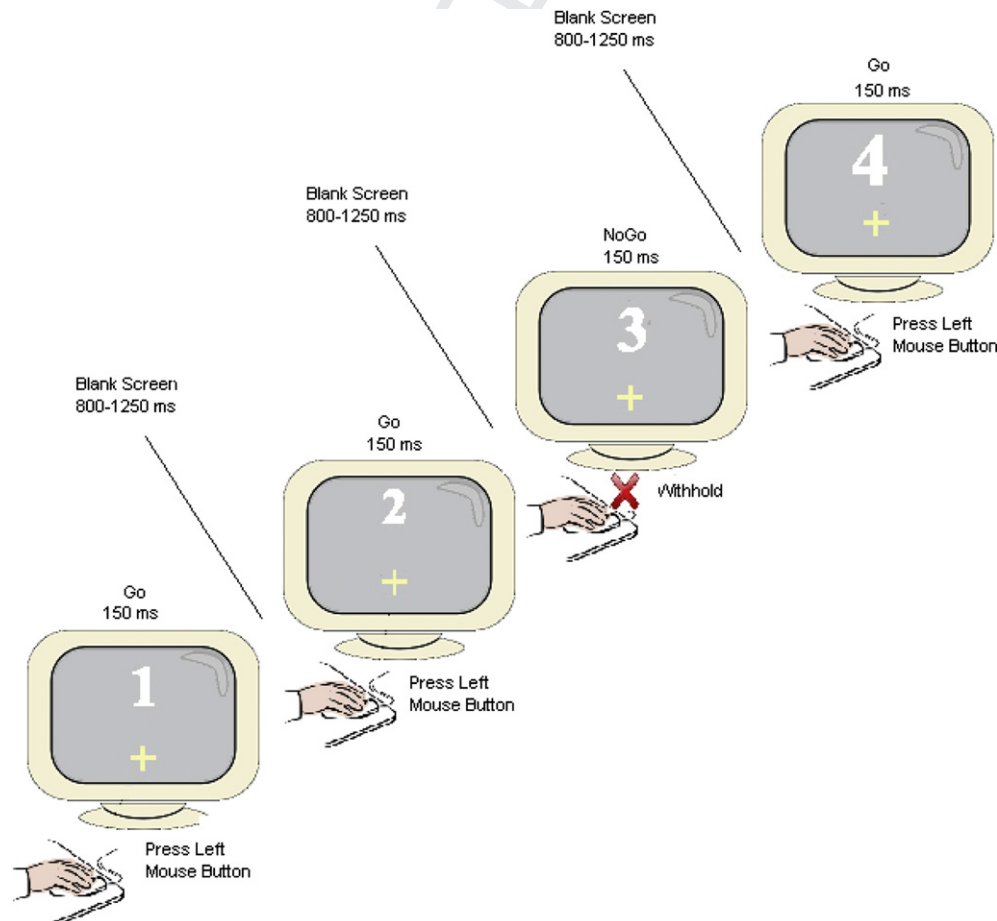
Fig. 1. The basic fixed-sequence SART paradigm is depicted schematically here. Subjects push a mouse button to each occurrence of a digit stimulus as the sequence cycles from 1 through 9, but they are required to withhold responding to occurrences of the digit "3".
