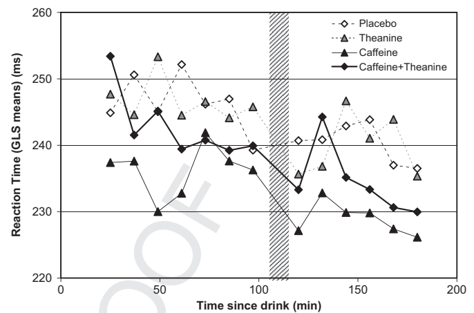
Fig. 5. Reaction times are plotted as a function of treatment and time. Caffeine decreased reaction times by 3% relative to placebo on average. There was no evidence of main or interaction effects involving theanine.
