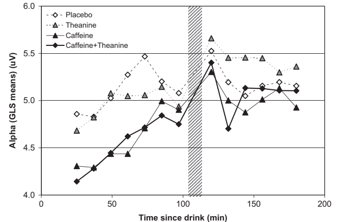
Fig. 6. Alpha-band activity is plotted as a function of treatment and time. Caffeine decreased alpha-band power. There were no main or interaction effects involving theanine.
