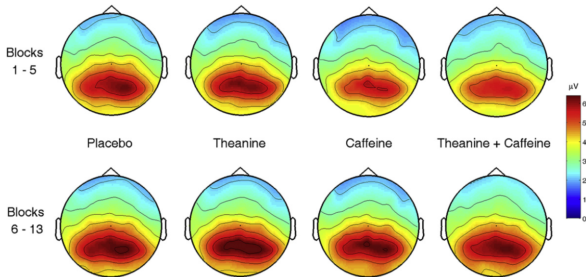
Fig. 7. Topographic maps of alpha-band activity during the 500-ms epoch preceding any digit stimulus showing that the suppression in the caffeine conditions was stronger in block 1–5 than in later blocks.
