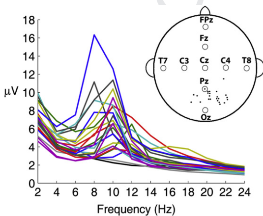
Fig. 2. Individual frequency spectra are plotted for each of the 21 participants from the scalp-site of maximal alpha-amplitude. The scalp-site of maximal alpha-amplitude is plotted on the inset cartoon head for each participant to illustrate the general parieto-occipital distribution of these maxima and the high inter-subject variability.
